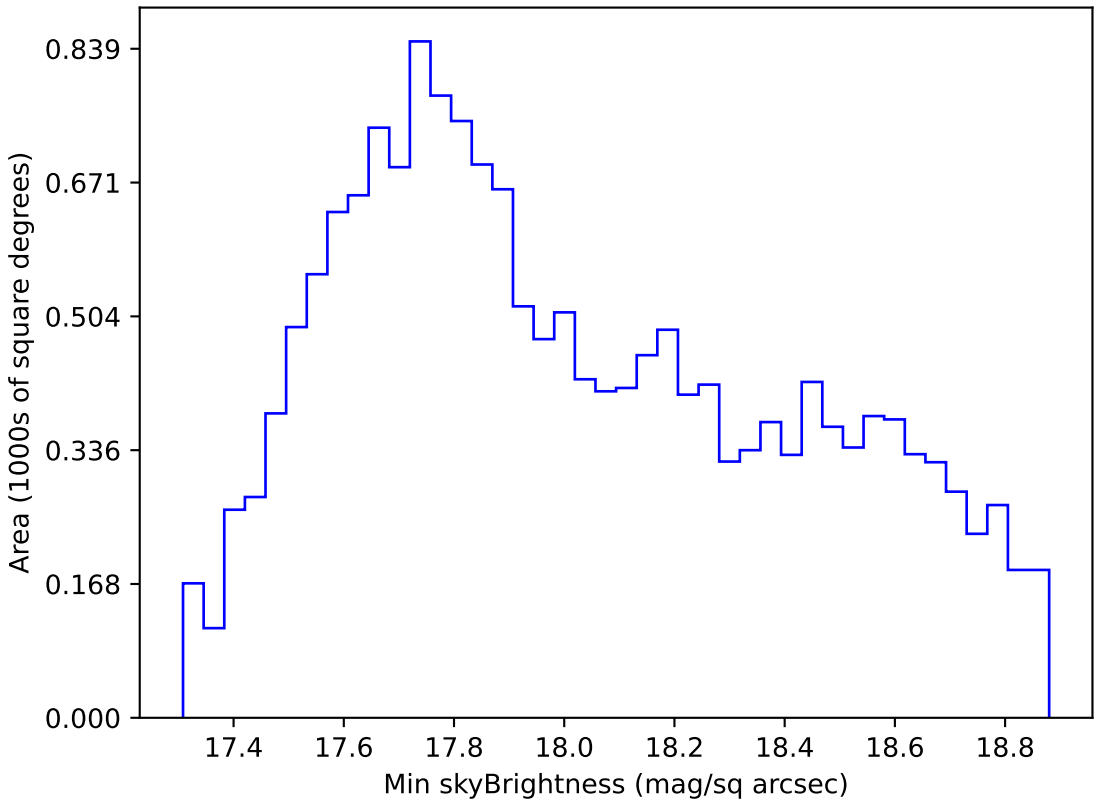
too_elab_r64_d2_ugrizy_v3.4_10yrs WFD i band: Min skyBrightness
