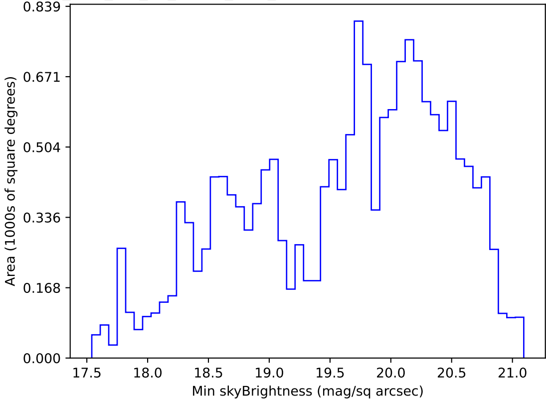
too_elab_r64_d2_ugrizy_v3.4_10yrs WFD g band: Min skyBrightness
