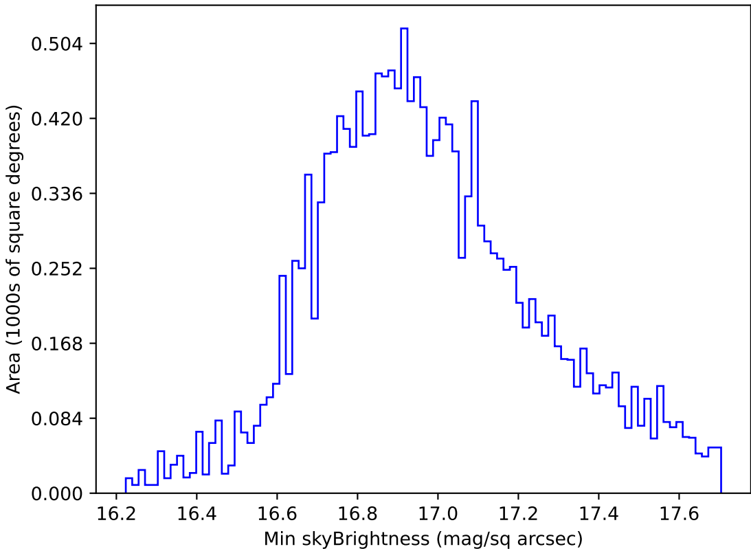
too_elab_r64_d2_ugrizy_v3.4_10yrs WFD all bands: Min skyBrightness
