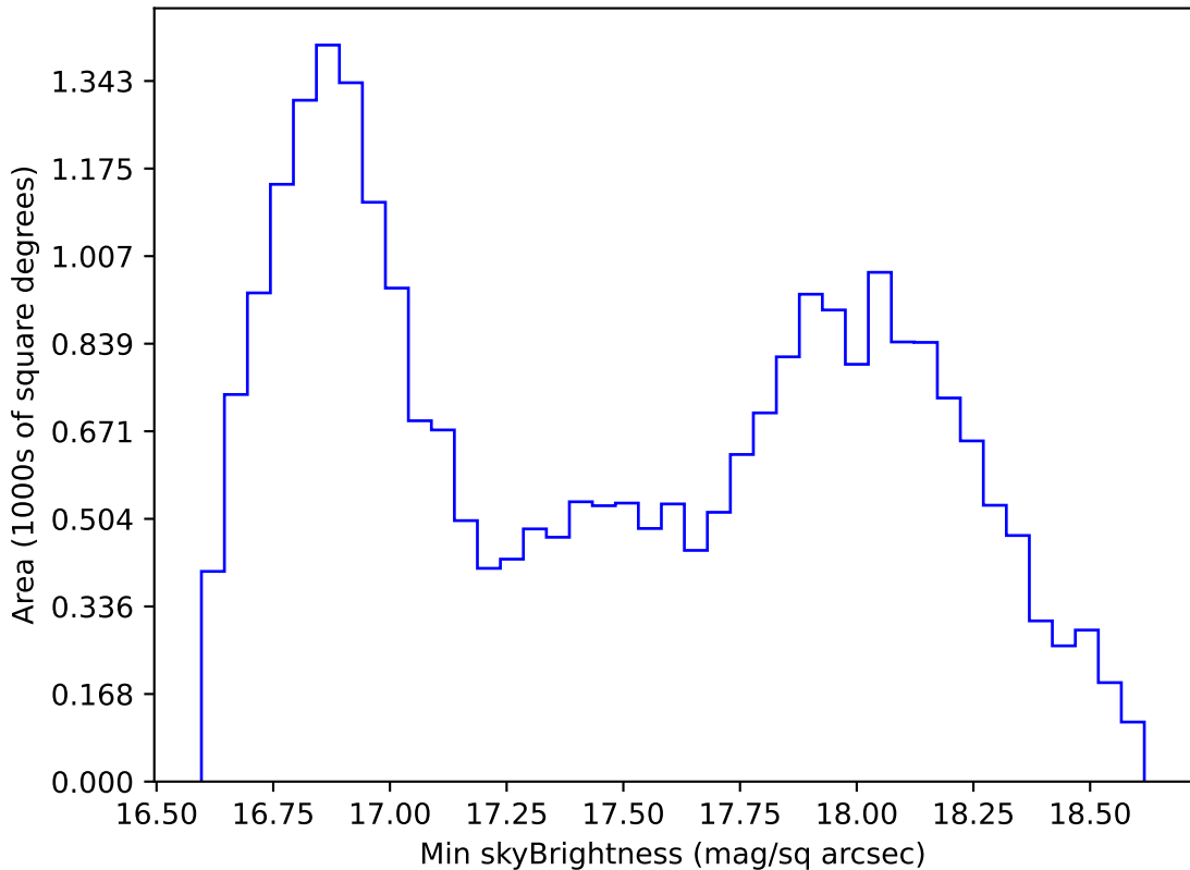
too_elab_r64_d2_ugrizy_v3.4_10yrs All sky z band: Min skyBrightness
