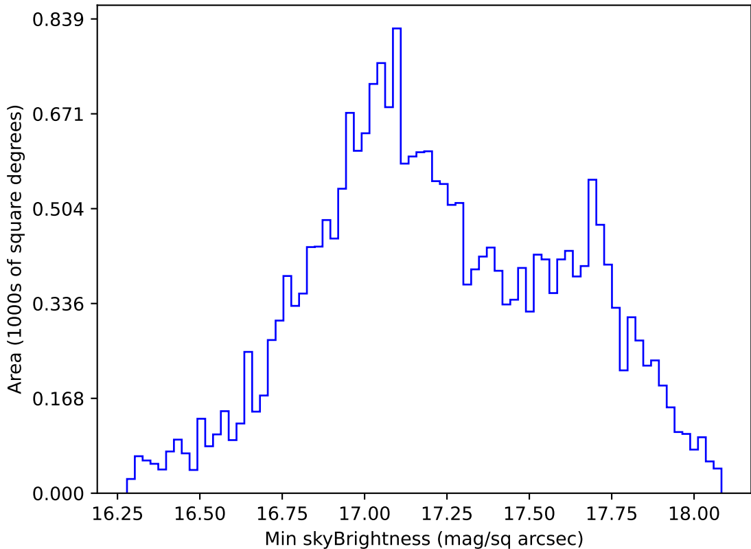
too_elab_r64_d2_ugrizy_v3.4_10yrs All sky y band: Min skyBrightness
