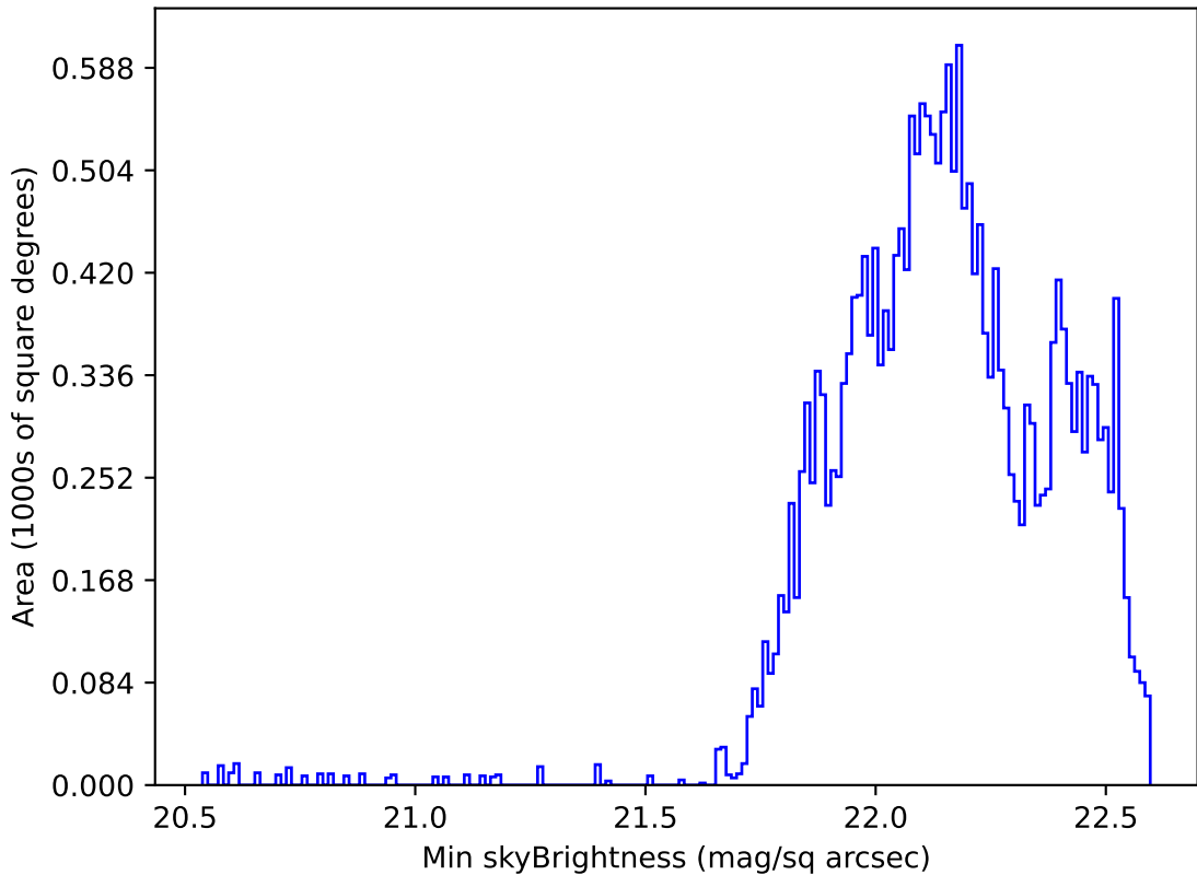
too_elab_r64_d2_ugrizy_v3.4_10yrs All sky u band: Min skyBrightness
