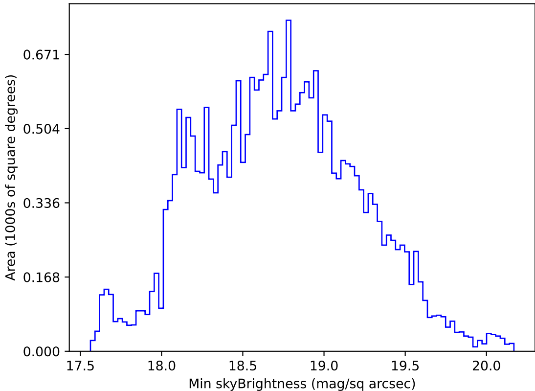
too_elab_r64_d2_ugrizy_v3.4_10yrs All sky r band: Min skyBrightness
