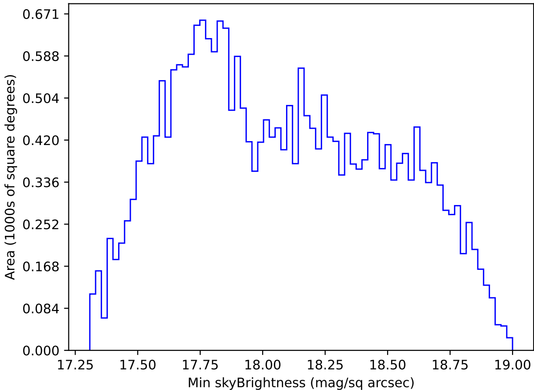
too_elab_r64_d2_ugrizy_v3.4_10yrs All sky i band: Min skyBrightness
