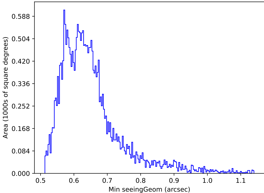
too_elab_r64_d2_ugrizy_v3.4_10yrs Yr 1 z band: Min seeingGeom
