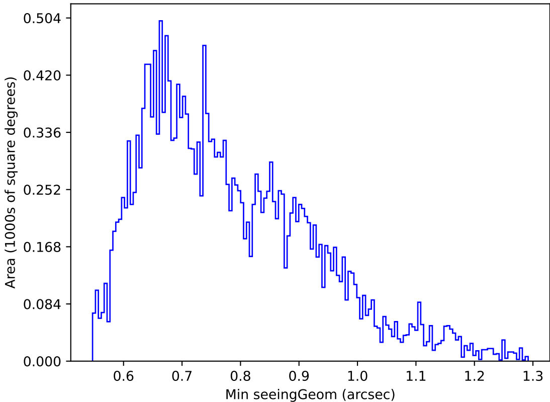
too_elab_r64_d2_ugrizy_v3.4_10yrs Yr 1 u band: Min seeingGeom
