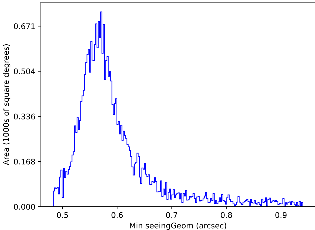
too_elab_r64_d2_ugrizy_v3.4_10yrs Yr 1 all bands: Min seeingGeom
