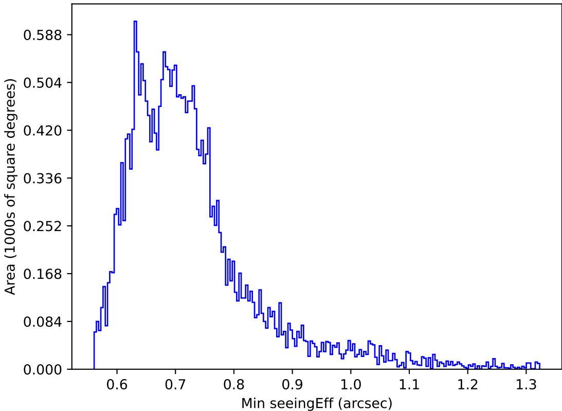
too_elab_r64_d2_ugrizy_v3.4_10yrs Yr 1 z band: Min seeingEff
