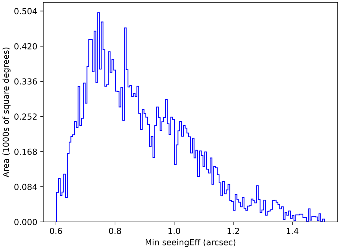
too_elab_r64_d2_ugrizy_v3.4_10yrs Yr 1 u band: Min seeingEff
