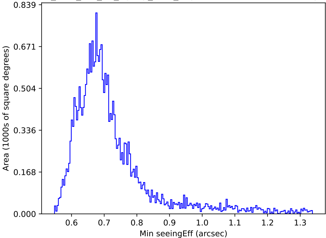
too_elab_r64_d2_ugrizy_v3.4_10yrs Yr 1 r band: Min seeingEff
