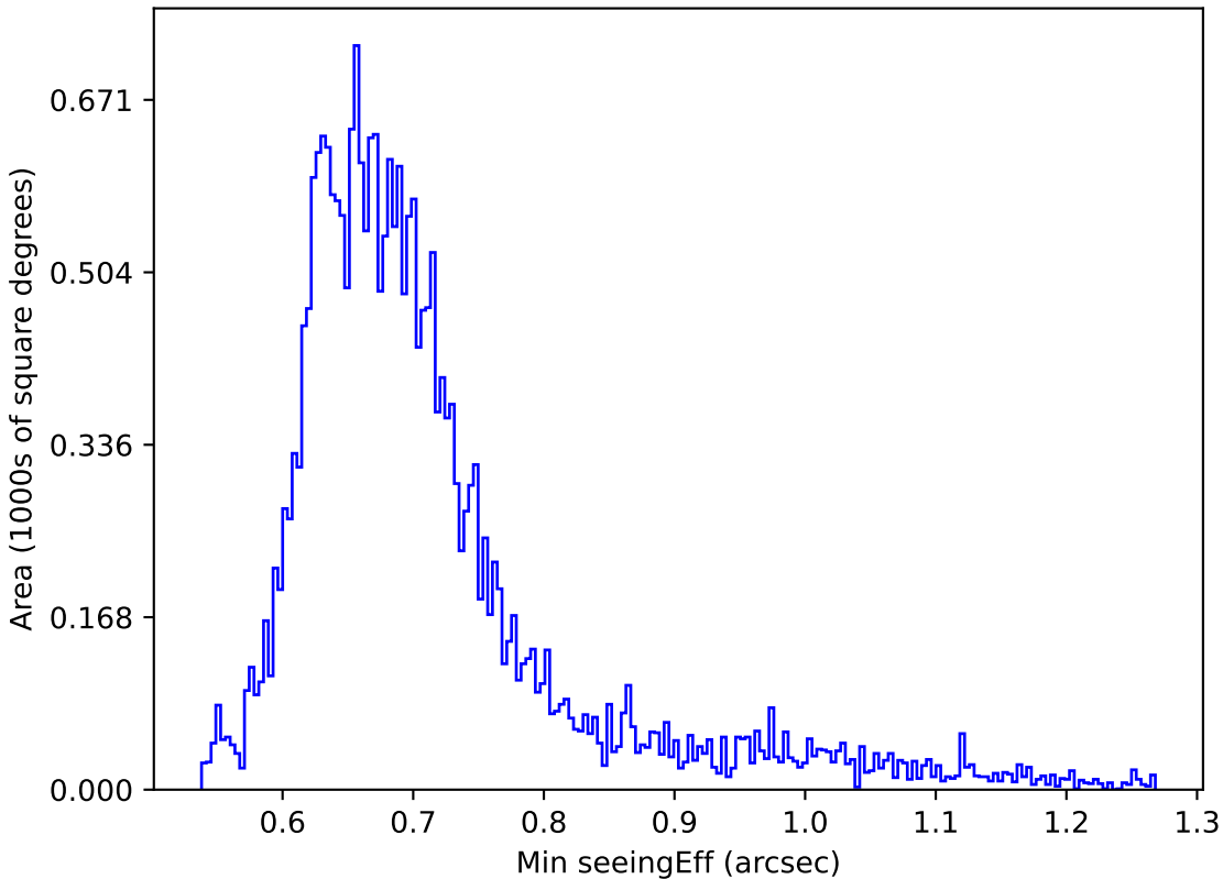
too_elab_r64_d2_ugrizy_v3.4_10yrs Yr 1 i band: Min seeingEff
