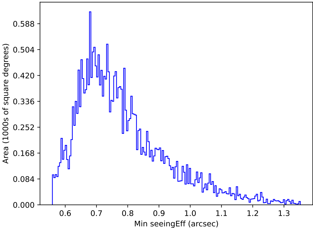
too_elab_r64_d2_ugrizy_v3.4_10yrs Yr 1 g band: Min seeingEff
