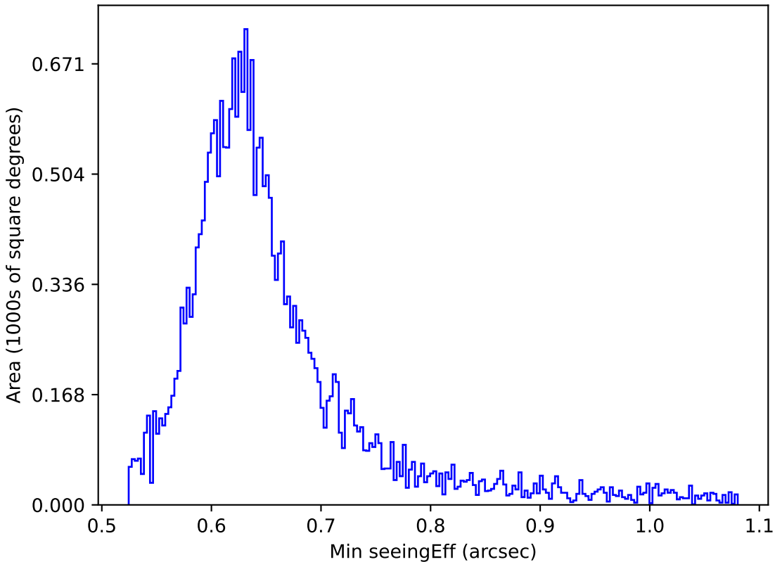
too_elab_r64_d2_ugrizy_v3.4_10yrs Yr 1 all bands: Min seeingEff
