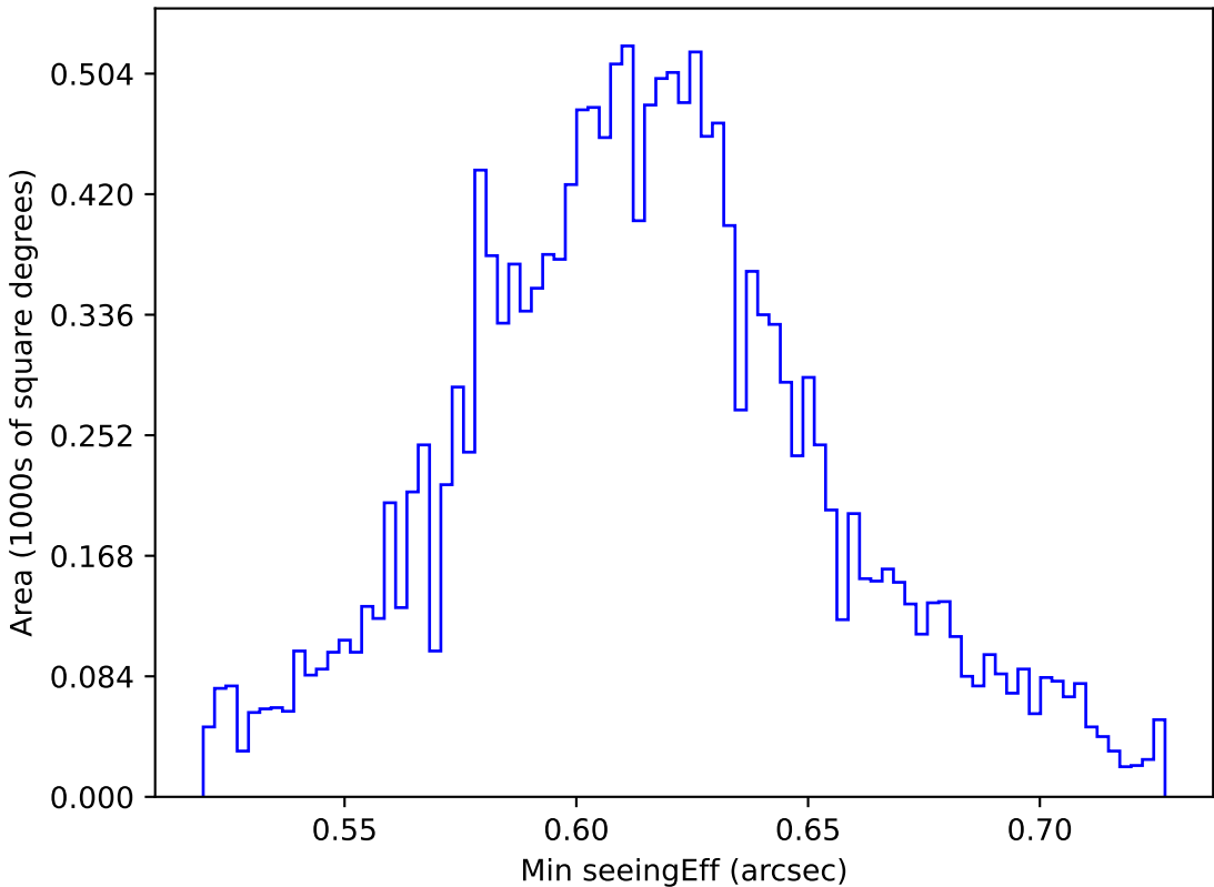
too_elab_r64_d2_ugrizy_v3.4_10yrs WFD z band: Min seeingEff
