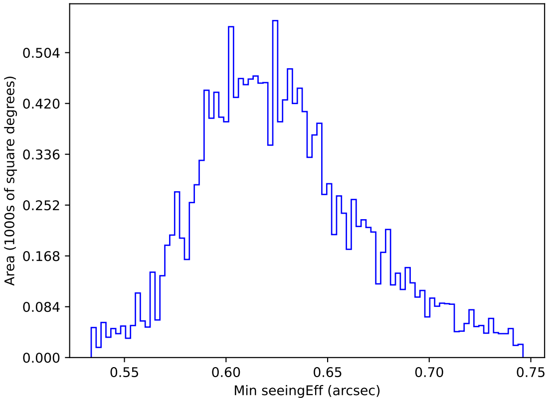
too_elab_r64_d2_ugrizy_v3.4_10yrs WFD y band: Min seeingEff
