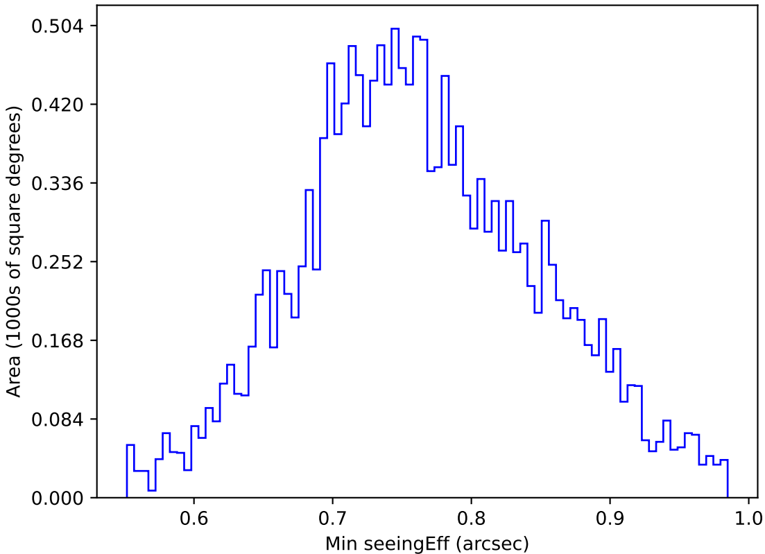
too_elab_r64_d2_ugrizy_v3.4_10yrs WFD u band: Min seeingEff
