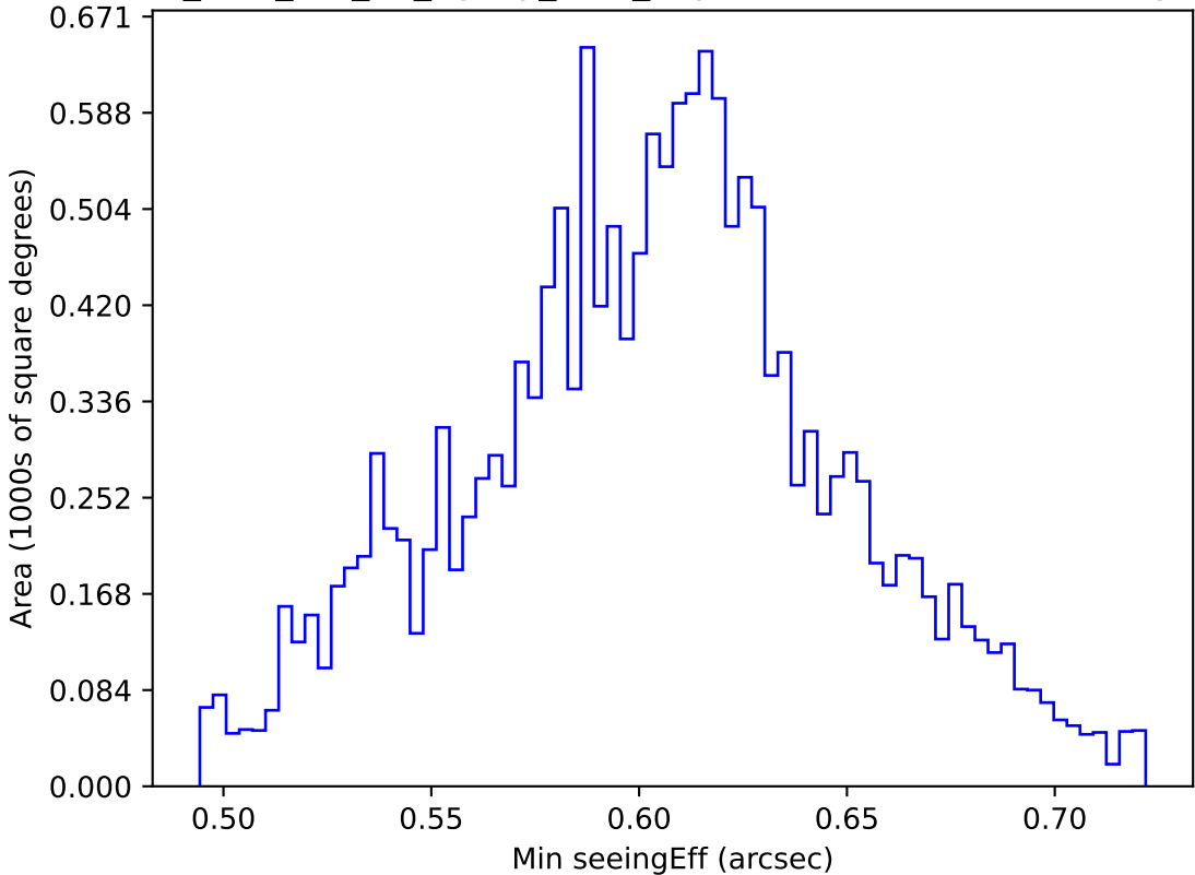
too_elab_r64_d2_ugrizy_v3.4_10yrs WFD i band: Min seeingEff
