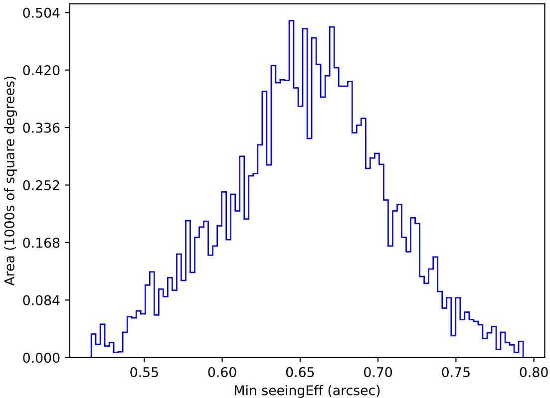
too_elab_r64_d2_ugrizy_v3.4_10yrs WFD g band: Min seeingEff
