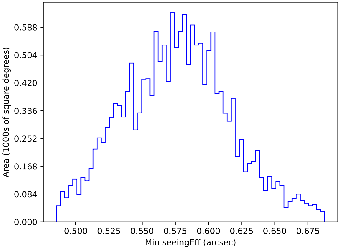
too_elab_r64_d2_ugrizy_v3.4_10yrs WFD all bands: Min seeingEff
