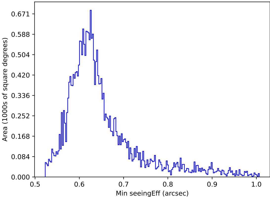
too_elab_r64_d2_ugrizy_v3.4_10yrs All sky z band: Min seeingEff
