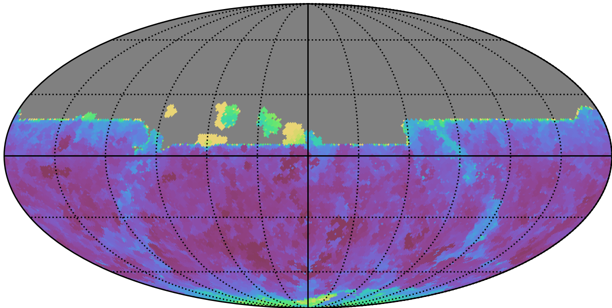
too_elab_r64_d2_ugrizy_v3.4_10yrs All sky y band: Min seeingEff
