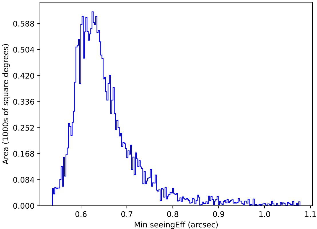
too_elab_r64_d2_ugrizy_v3.4_10yrs All sky y band: Min seeingEff
