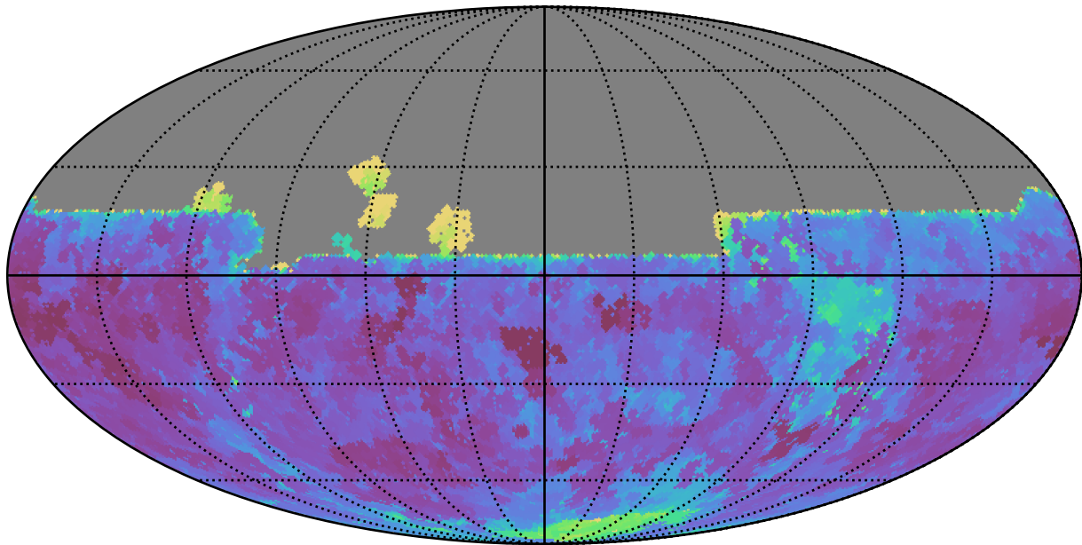
too_elab_r64_d2_ugrizy_v3.4_10yrs All sky u band: Min seeingEff
