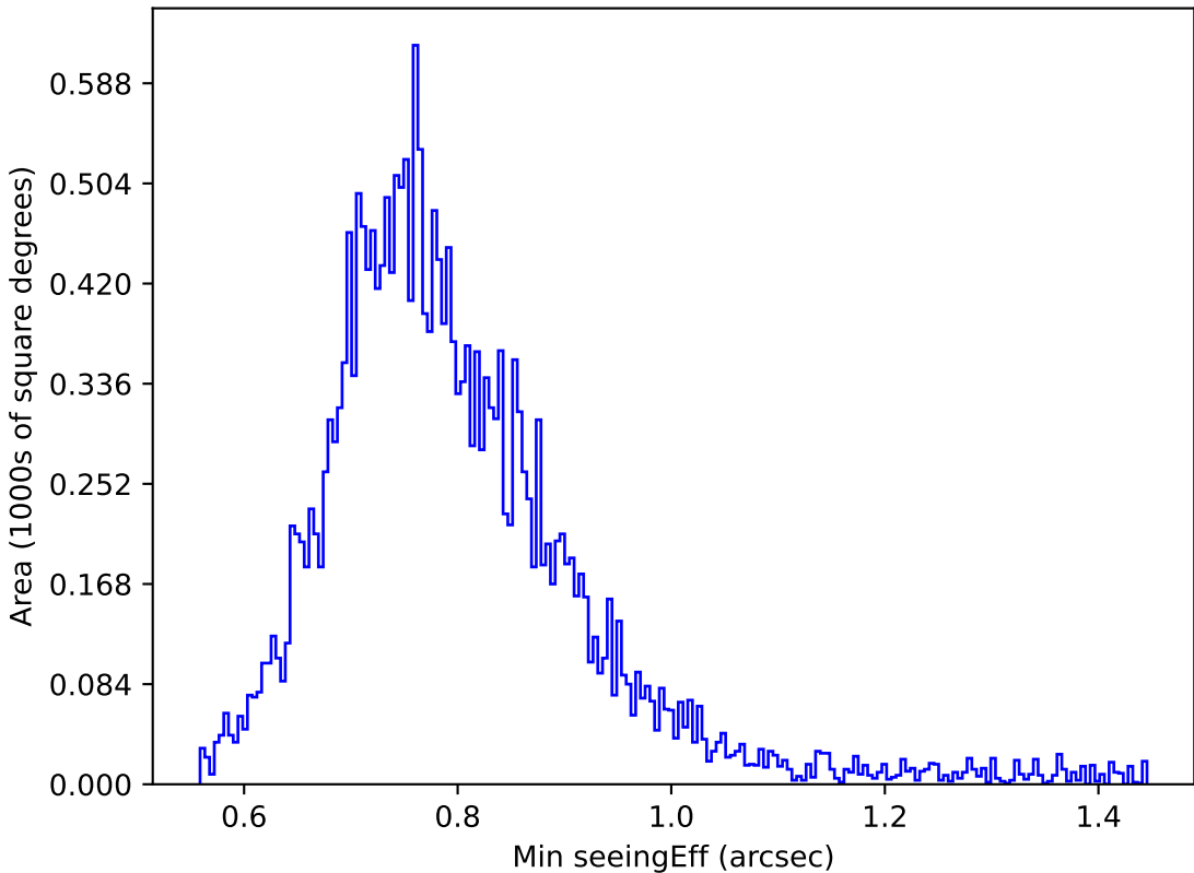
too_elab_r64_d2_ugrizy_v3.4_10yrs All sky u band: Min seeingEff
