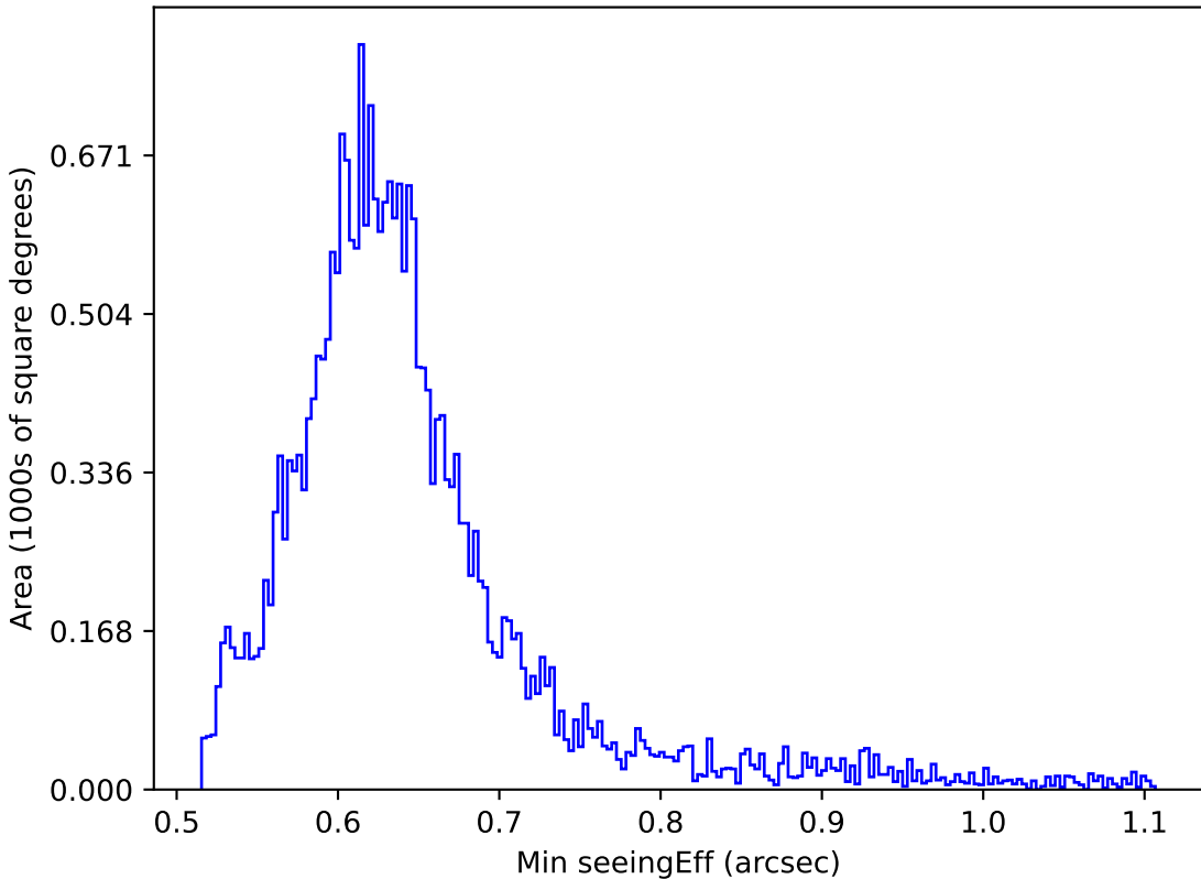
too_elab_r64_d2_ugrizy_v3.4_10yrs All sky r band: Min seeingEff
