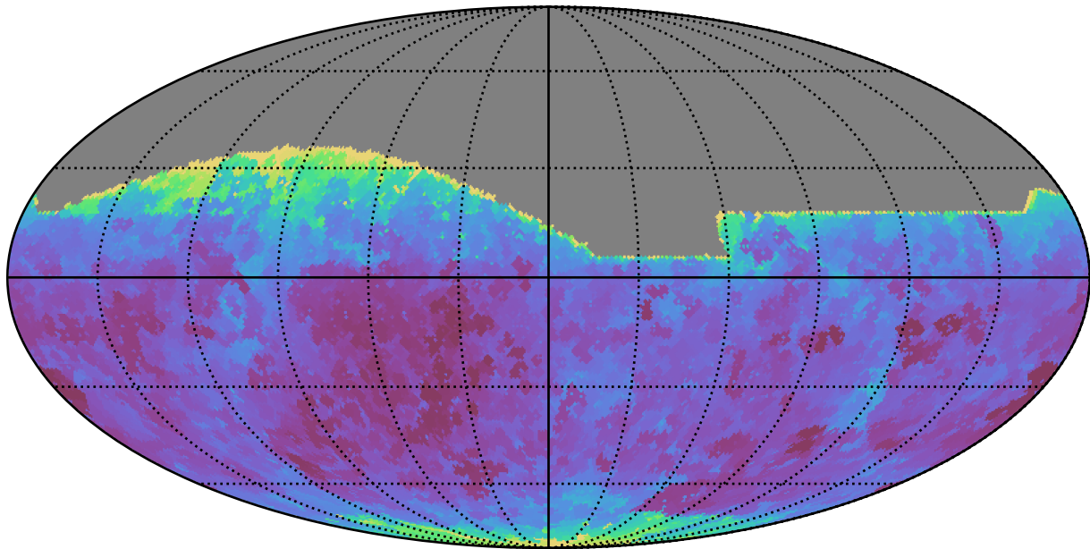
too_elab_r64_d2_ugrizy_v3.4_10yrs All sky i band: Min seeingEff
