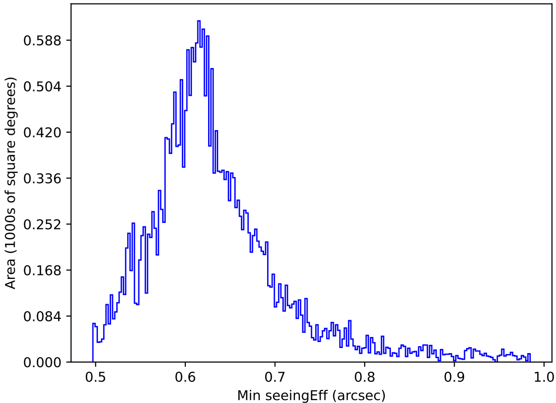
too_elab_r64_d2_ugrizy_v3.4_10yrs All sky i band: Min seeingEff
