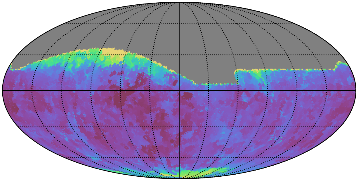
too_elab_r64_d2_ugrizy_v3.4_10yrs All sky g band: Min seeingEff
