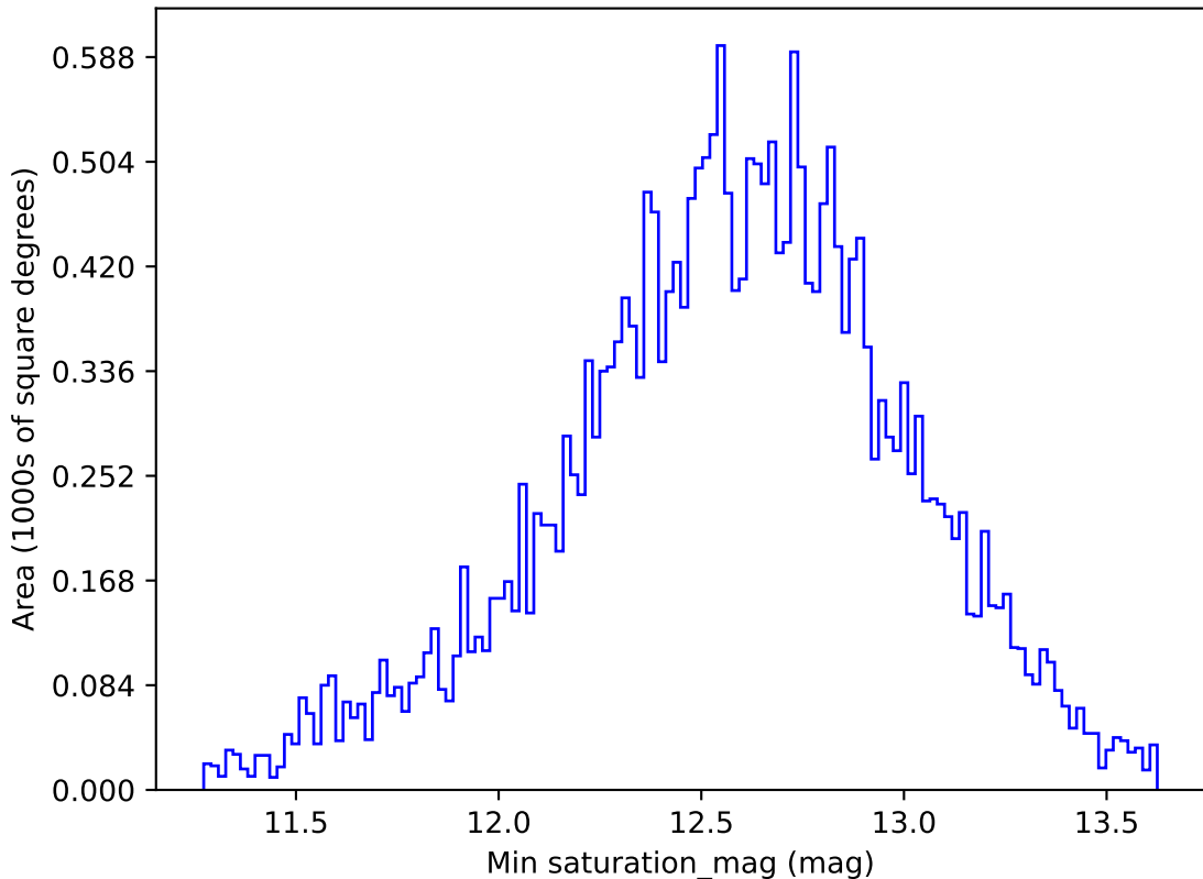
too_elab_r64_d2_ugrizy_v3.4_10yrs All sky r band: Min saturation_mag
