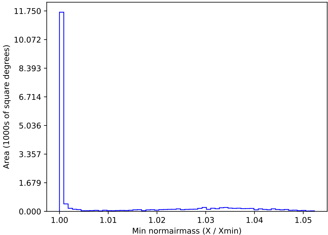
too_elab_r64_d2_ugrizy_v3.4_10yrs WFD u band: Min normairmass
