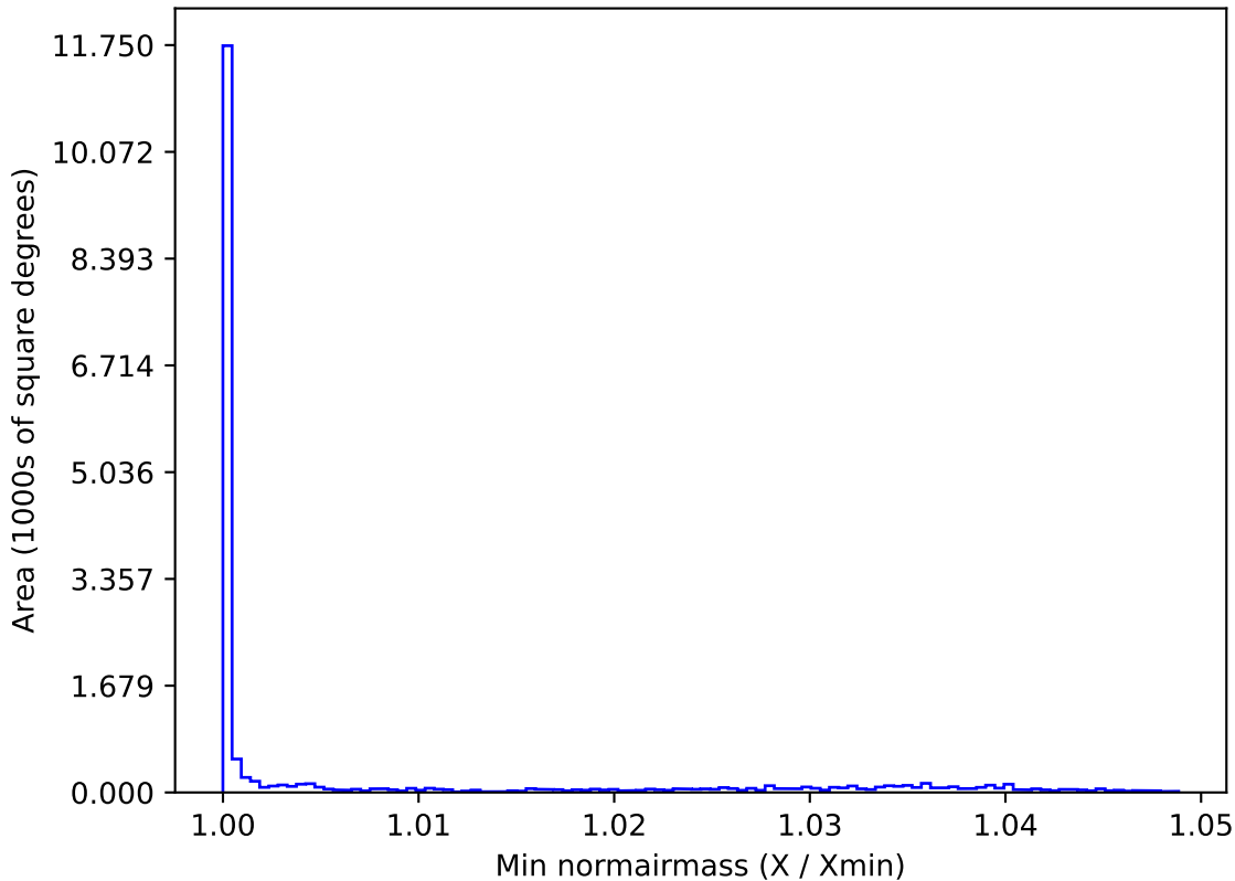
too_elab_r64_d2_ugrizy_v3.4_10yrs WFD g band: Min normairmass
