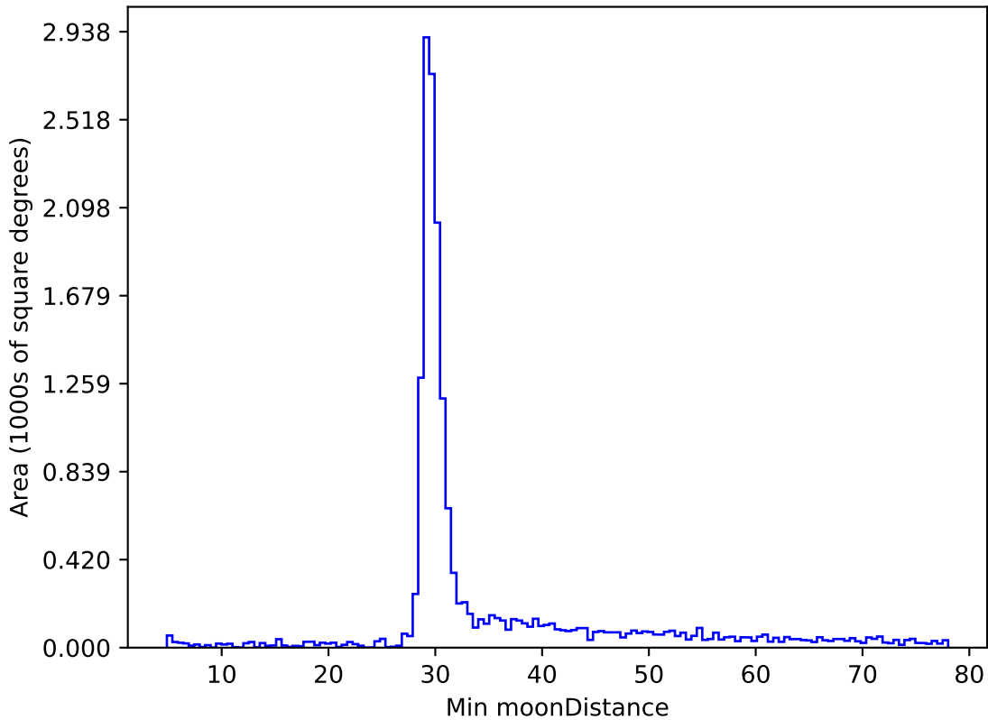
too_elab_r64_d2_ugrizy_v3.4_10yrs WFD z band: Min moonDistance
