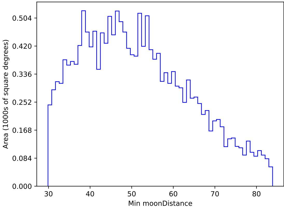
too_elab_r64_d2_ugrizy_v3.4_10yrs WFD u band: Min moonDistance
