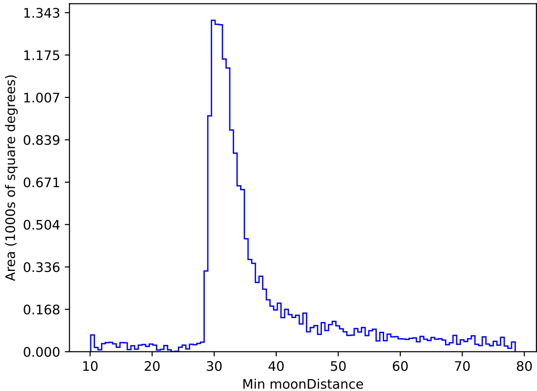
too_elab_r64_d2_ugrizy_v3.4_10yrs WFD r band: Min moonDistance
