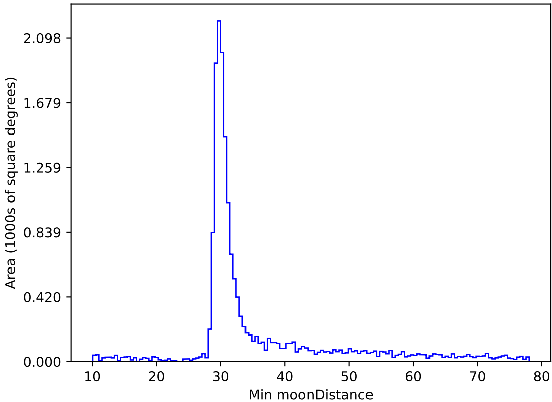
too_elab_r64_d2_ugrizy_v3.4_10yrs WFD i band: Min moonDistance
