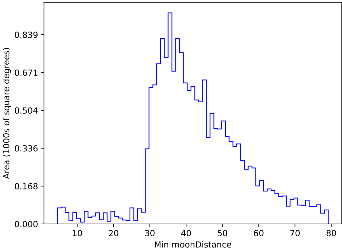
too_elab_r64_d2_ugrizy_v3.4_10yrs WFD g band: Min moonDistance
