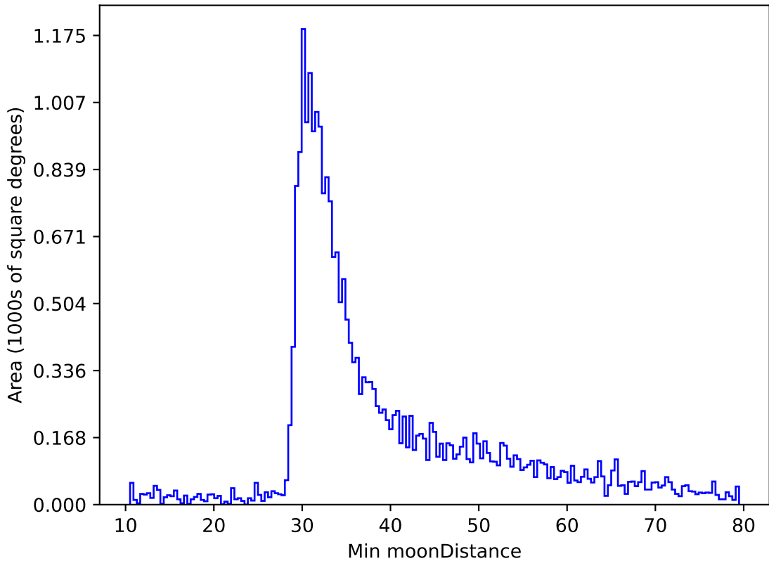
too_elab_r64_d2_ugrizy_v3.4_10yrs All sky r band: Min moonDistance
