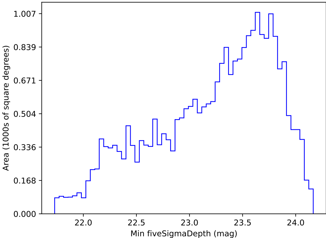
too_elab_r64_d2_ugrizy_v3.4_10yrs Yr 1 r band: Min fiveSigmaDepth
