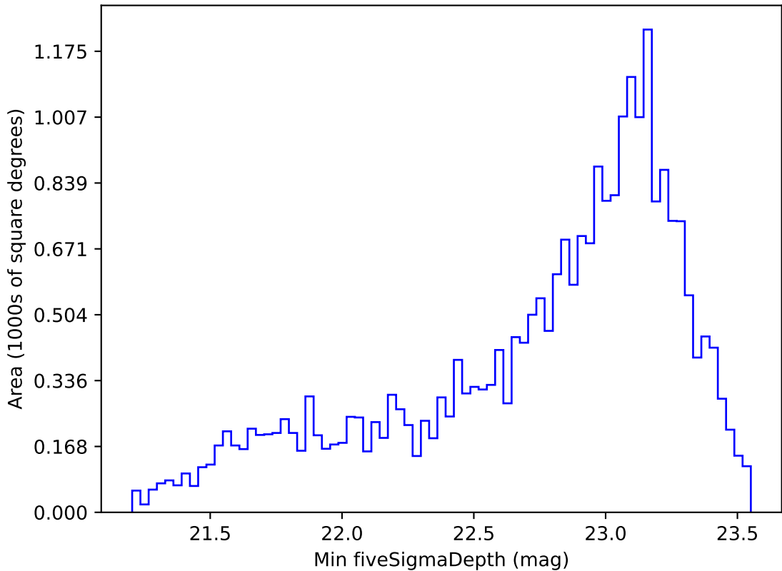
too_elab_r64_d2_ugrizy_v3.4_10yrs Yr 1 i band: Min fiveSigmaDepth
