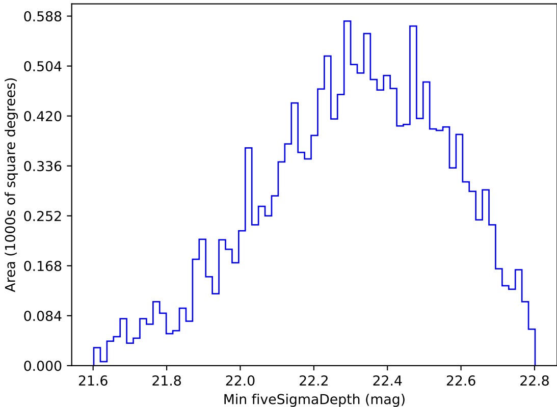
too_elab_r64_d2_ugrizy_v3.4_10yrs WFD u band: Min fiveSigmaDepth
