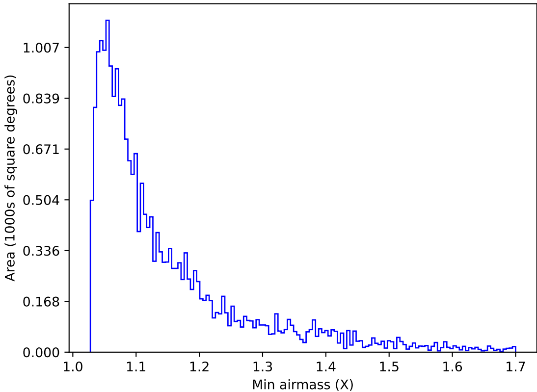
too_elab_r64_d2_ugrizy_v3.4_10yrs Yr 1 u band: Min airmass
