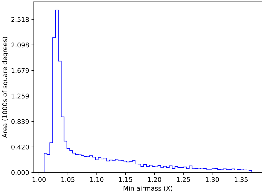
too_elab_r64_d2_ugrizy_v3.4_10yrs WFD y band: Min airmass
