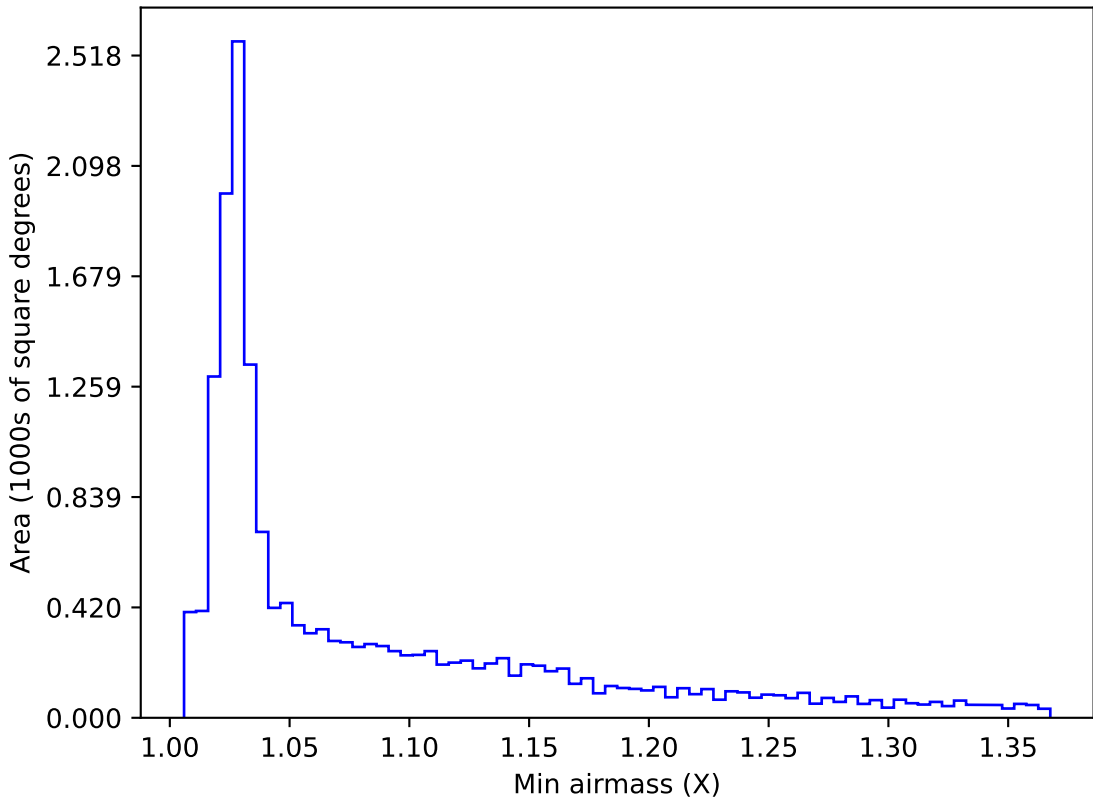
too_elab_r64_d2_ugrizy_v3.4_10yrs WFD r band: Min airmass
