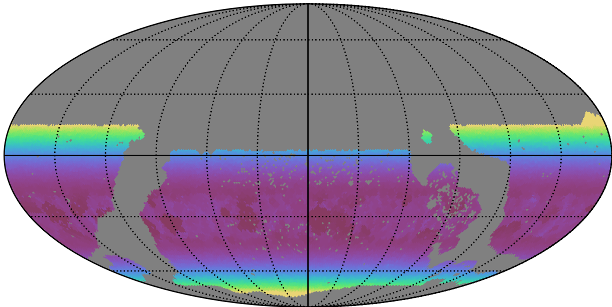
too_elab_r64_d2_ugrizy_v3.4_10yrs WFD g band: Min airmass
