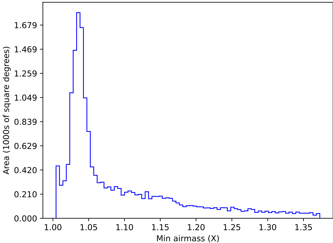
too_elab_r64_d2_ugrizy_v3.4_10yrs WFD g band: Min airmass
