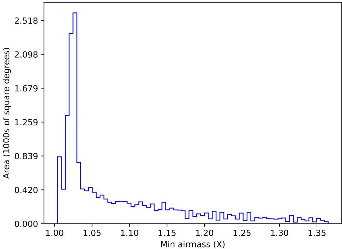
too_elab_r64_d2_ugrizy_v3.4_10yrs WFD all bands: Min airmass
